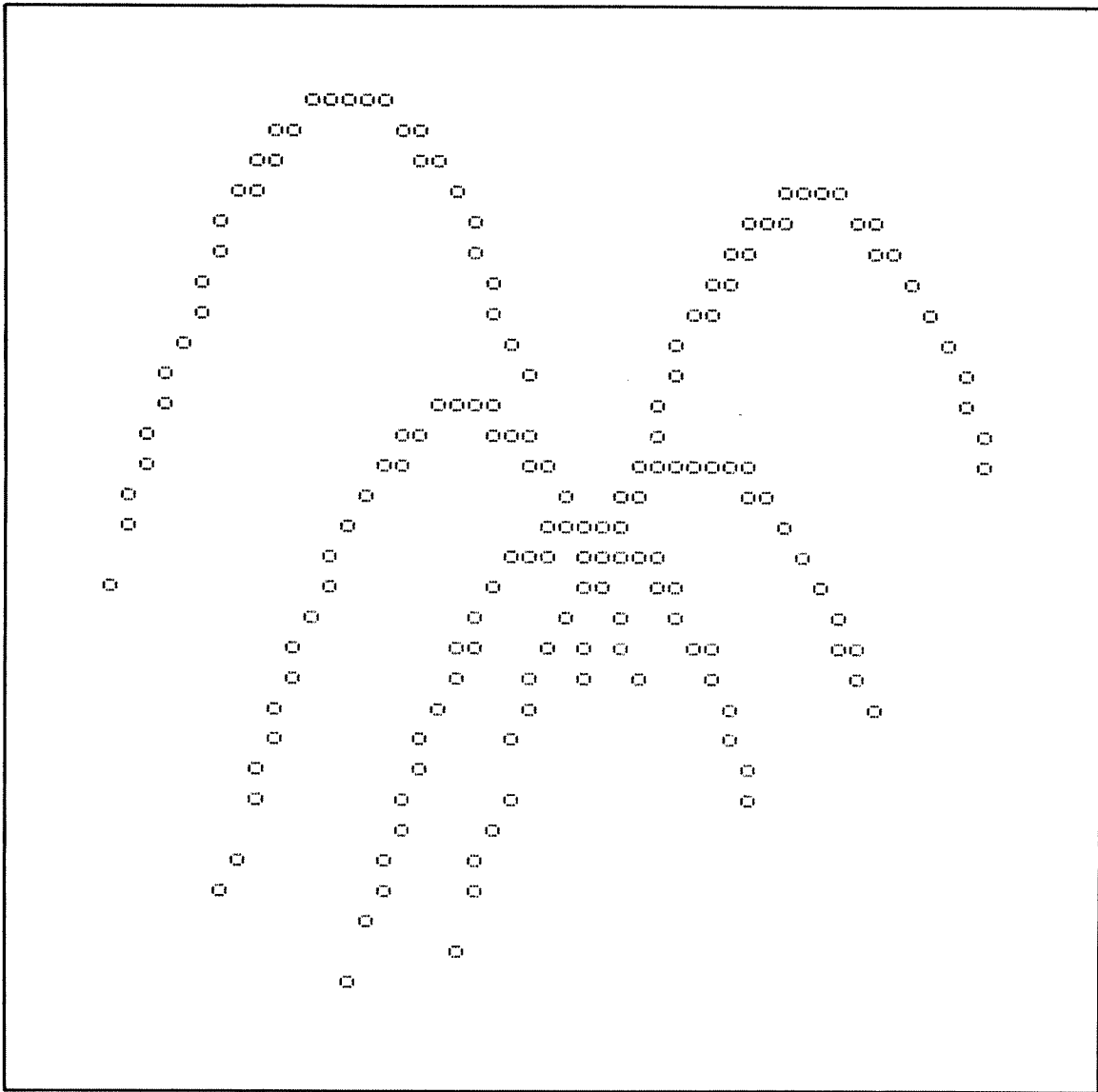
Fig. 3-1. The function Z=X*X-Y*Y , a saddle-shaped figure.
