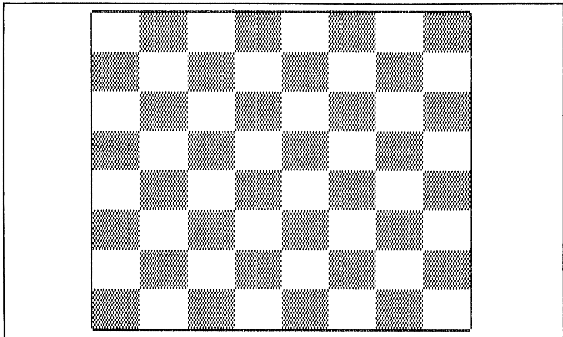
Fig. 6-2. A chessboard.
